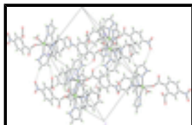
Fig. 2. Crystal packing of the title compound, displayed with hydrogen bonds as dashed lines.
